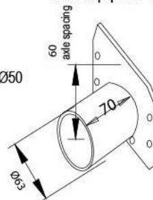
Art. FC92.63 Outlet cap flange with HORIZONTAL outlet pipe Ø 63 mm
