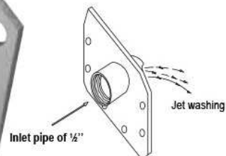
Art. FC92M Inlet cap flange with pipe coupling of 1/2"
