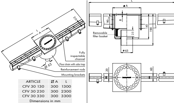
STAINLESS STEEL SLOT CHANNELS WITH ODOR TRAP AND REMOVABLE FILTER BASKET CENTRAL VERTICAL OUTLET
