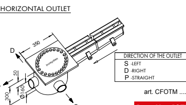
END HORIZONTAL OUTLET
