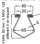
SLOT CHANNEL CROSS SECTION Art. Inoxsystem® -C2-
