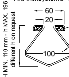
SLOT CHANNEL CROSS SECTION Art. Inoxsystem® -MC2-
