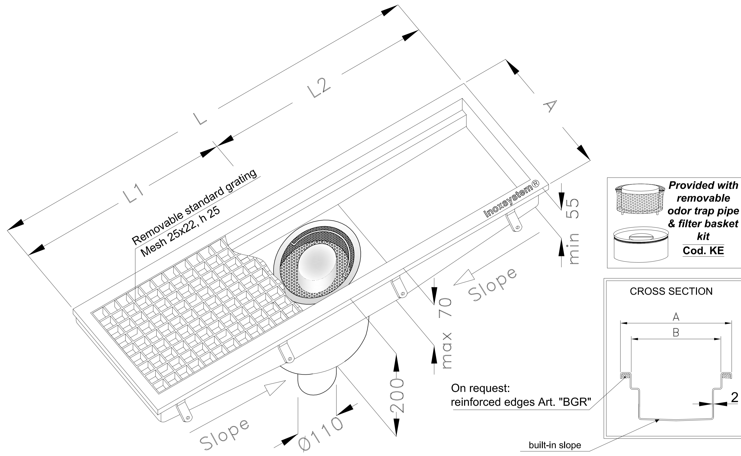
Grade 304 stainless steel (grade 316L on request) - Sheet thk. 2 mm
